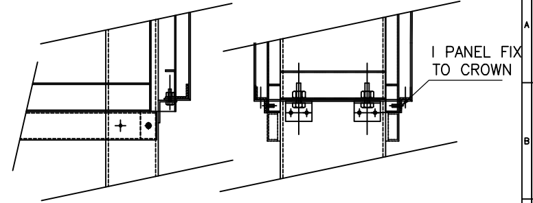
DETAIL AT Z CROWN FRAME ASSY.
