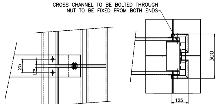
DETAIL AT Y
