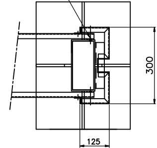
DETAIL AT X
